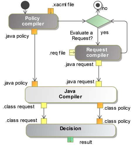
Figure 5: FACPL Policy Decision Point
