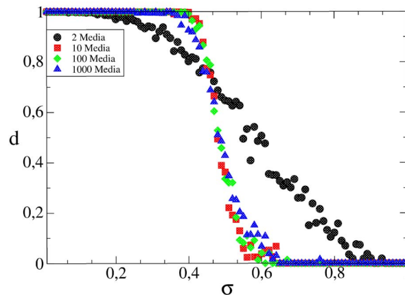
Figure 2 | Maximal opinion distance d (the difference between the highest and lowest opinion in the gossipers' network) versus tolerance \sigma . The size of the symbols is bigger than the error bars. Opinions' distance under the effect of audience-oriented unpolarized media shows a smoothing of the transition (less sharp change of d versus \sigma ).
