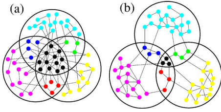
FIG. 1. (Color online) Schematic network snapshots of the BBS network (a) and traditional social network (b).
