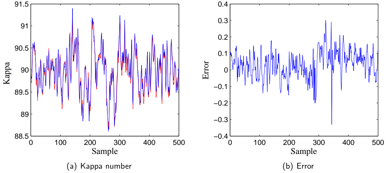
Figure 4: Hardwood/Kappa number = 90; Nonparametric LPV identification ( open-loop ): (a) true Kappa number (blue), estimated Kappa number (red); (b) difference between true Kappa number and estimated Kappa number.
