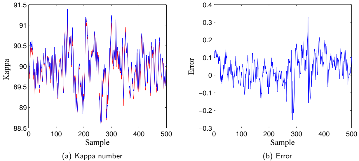
Figure 5: Hardwood/Kappa number = 90; Nonparametric LPV identification ( closed-loop ): (a) true Kappa number (blue), estimated Kappa number (red); (b) difference between true Kappa number and estimated Kappa number.
