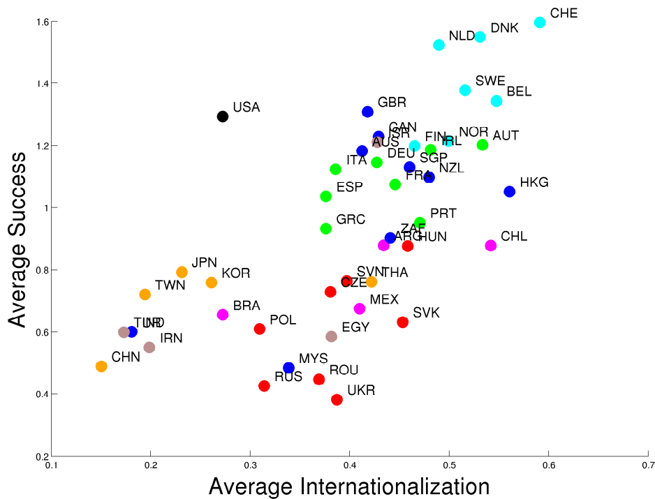
FIG. 1. Relation between average internationalization \bar{\mathcal{I}} and average scientific success \bar{\mathcal{S}} of nations.
