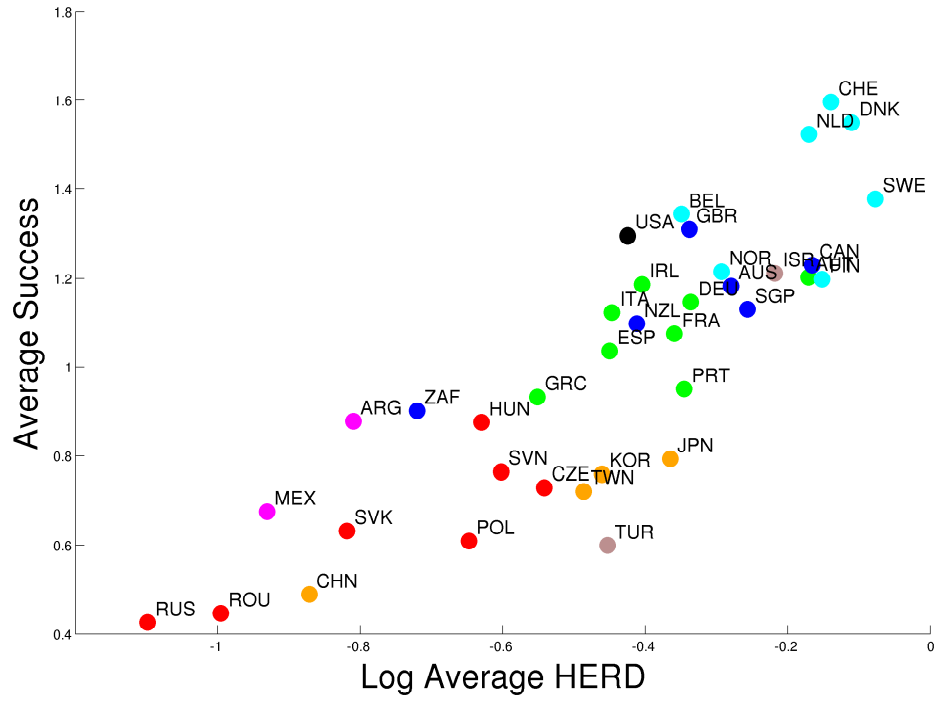
FIG. 5. Relation between average HERD \bar{H} and average scientific success \bar{S} of nations.
