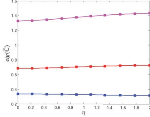
Figure 5: Eigenvalues of \tilde{\mathbf{C}} vs the piezo-electric multiplicative factor \eta .
