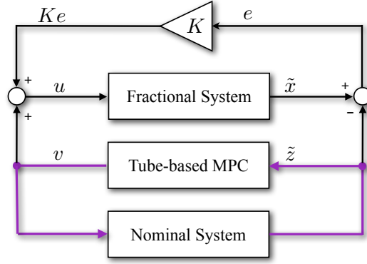
Fig. 1: Tube-based MPC for fractional order systems. The nominal system is a finite dimension LTI system in discrete-time.
